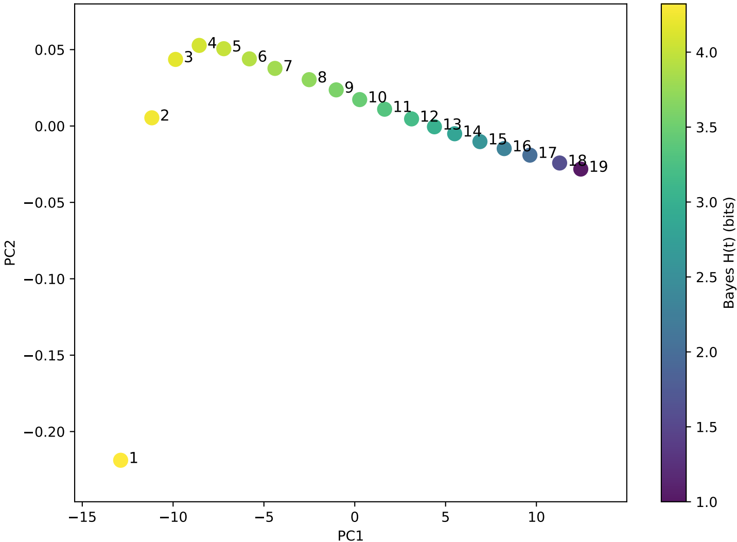
Value Manifold (PCA of pooled final representation)
